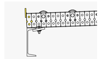
BKE Clamping clip with screw
